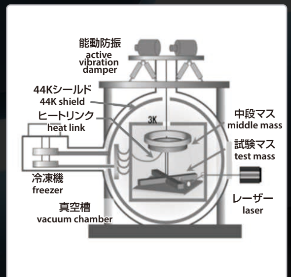
低温ねじれ振り子型重力勾配計 Low-temp torsion pendulum gravity gradient meter
